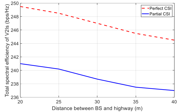
Fig. 6. Total spectral efficiency of the V2Is versus the distance between the BS and highway.
