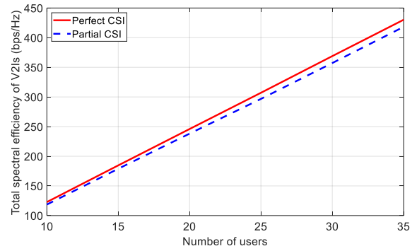
Fig. 5. Total spectral efficiency versus the number of V2Is.
