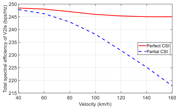
Fig. 4. Total spectral efficiency of the V2Is versus different velocity.
