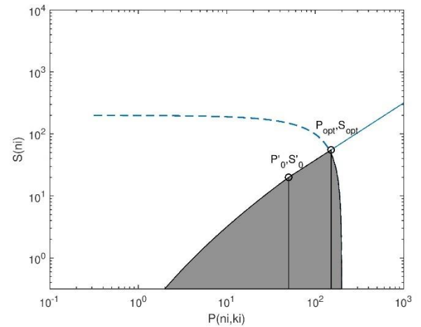
(c) Feasible region in case II
