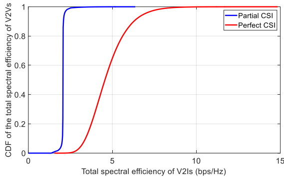
Fig. 3. CDF of the total spectral efficiency of a V2V.
