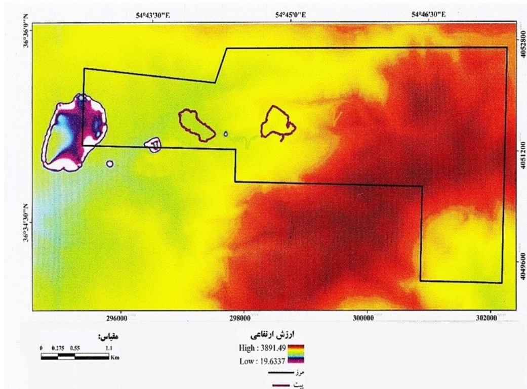
Fig 2. Map of elevation dispersal of the study area
